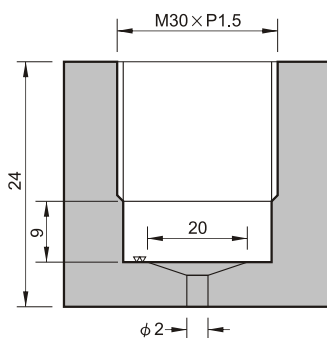
Mounting diagram
