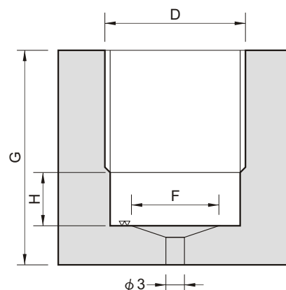
Mounting diagram
