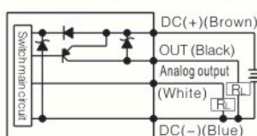
RL5□-031-□-□ PNP+Analog(Current)output
