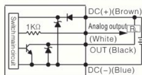
RL5□-030-□-□ NPN+Analog(Voltage)output
